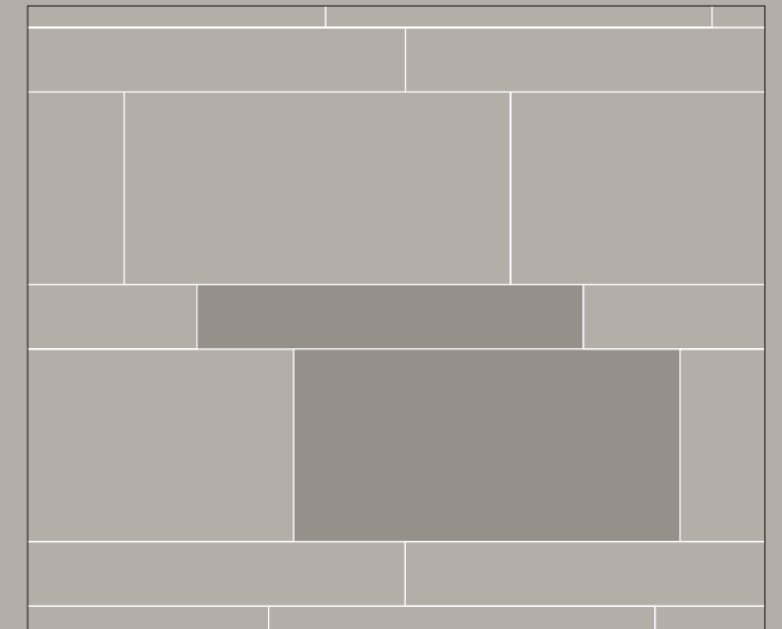
60x120 (24"x48") RT - 80,00% 20x120 (8"x48") RT - 20,00%
