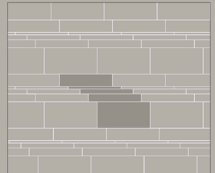
30x60 (12"x24") RT - 46,94% 6,4x60 (2 1 / 2 "x24") RT - 10,03% 14,7x60 (5 3 / 4 "x24") RT - 23,00% 3,1x60 (1 1 / 4 "x24") RT - 4,84% 9,7x60 (3 7 / 8 "x24") RT - 15,18%
